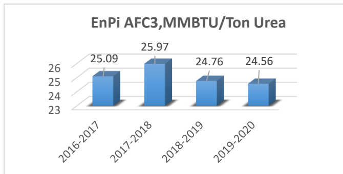
Figure 5. AFC III Energy Performance Indicator
